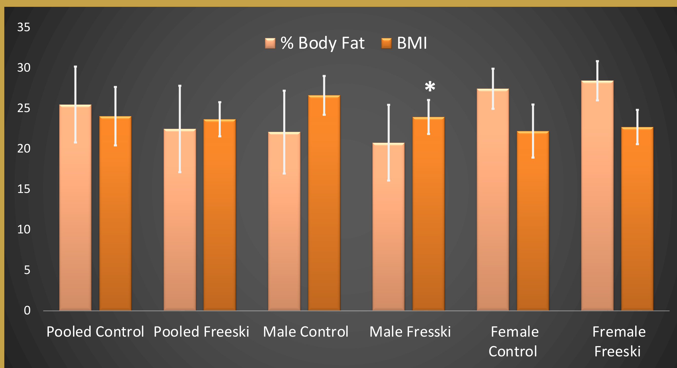
Figure 1: Percent body fat and BMI (kg/m 2 ) of pooled (male and female) freeski and nonfreeski athletes. Bars denote standard deviations. Star (*) denotes statistical significance.
